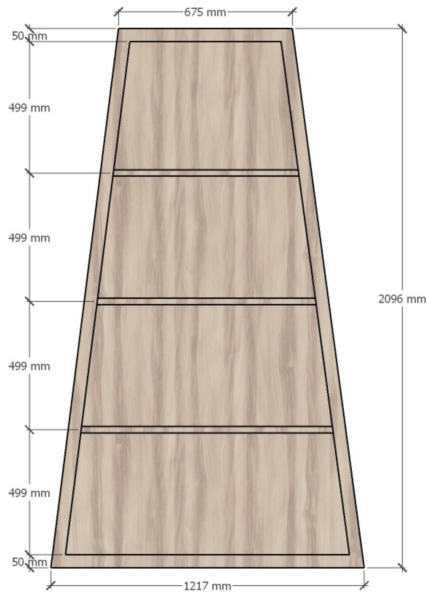
Front Elevation
