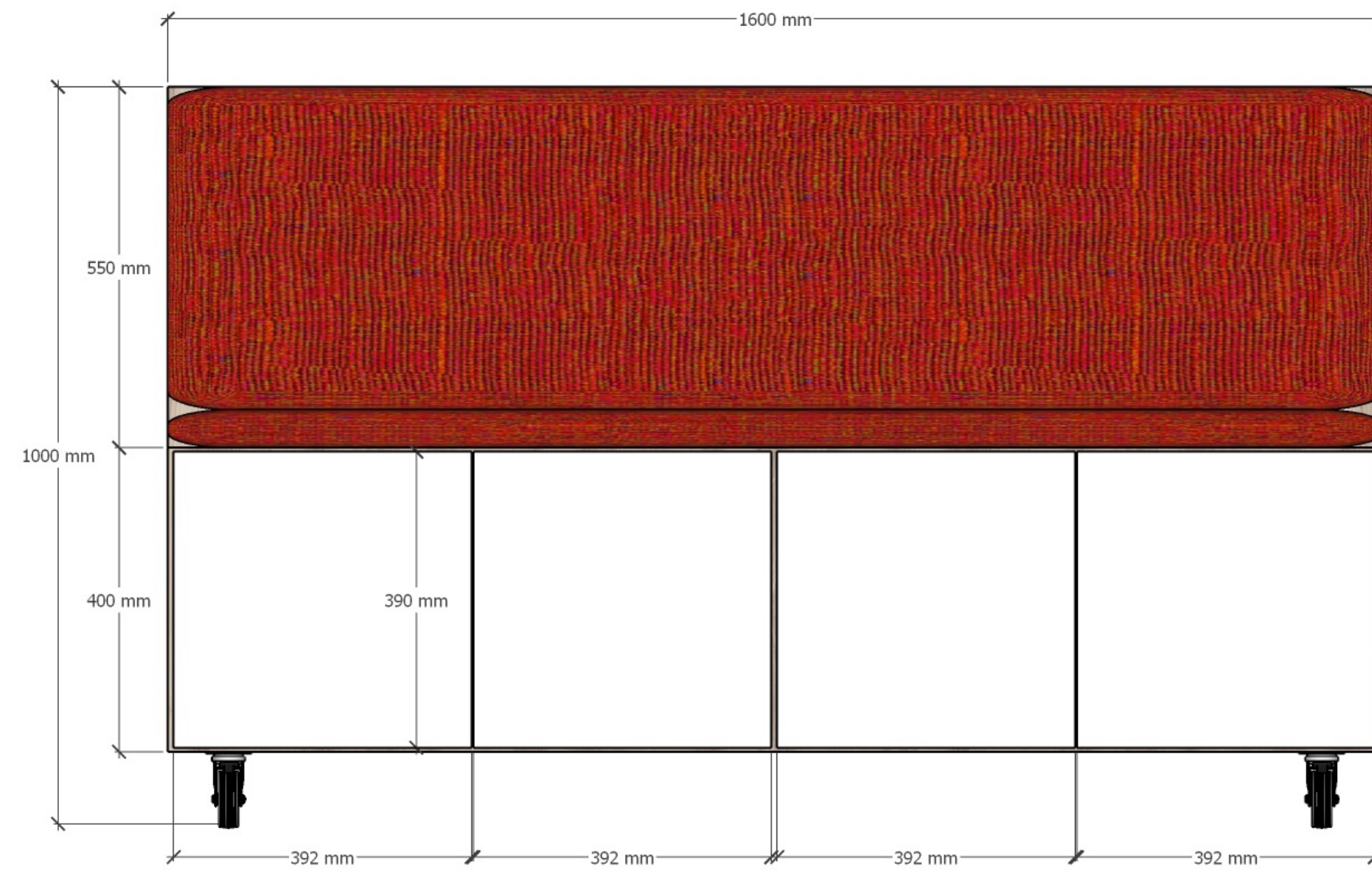
Front Elevation
