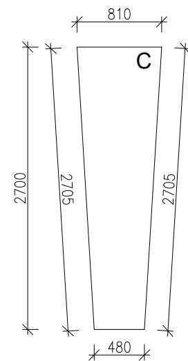
6 PANEL C 802 SCALE 1:50
