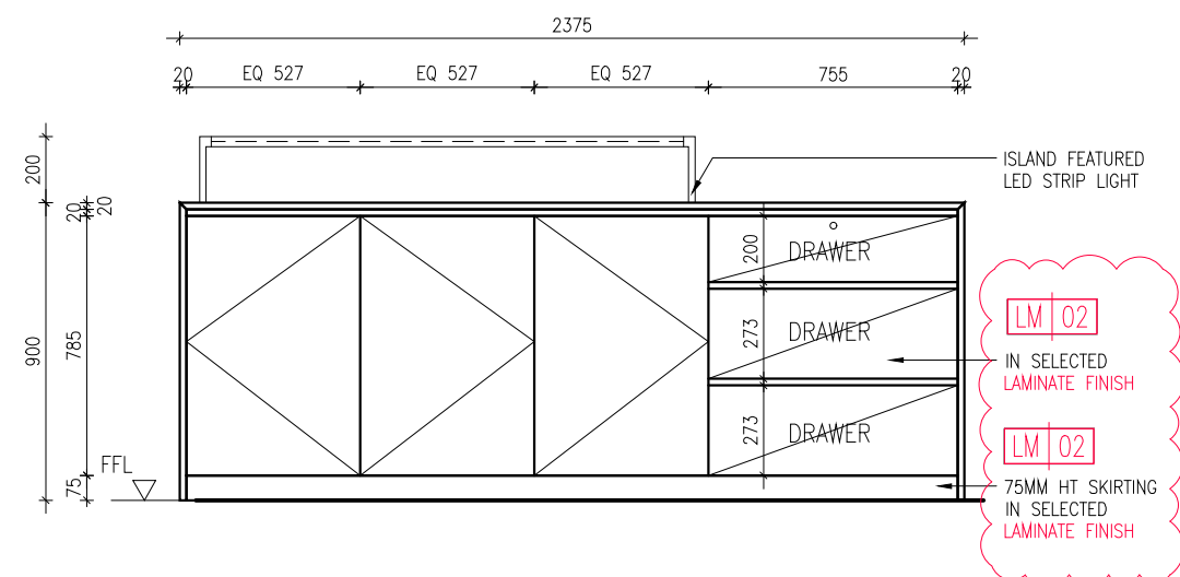
04 605 CAFÉ - FEATURE ISLAND - ELEVATION 2 SCALE 1:25
