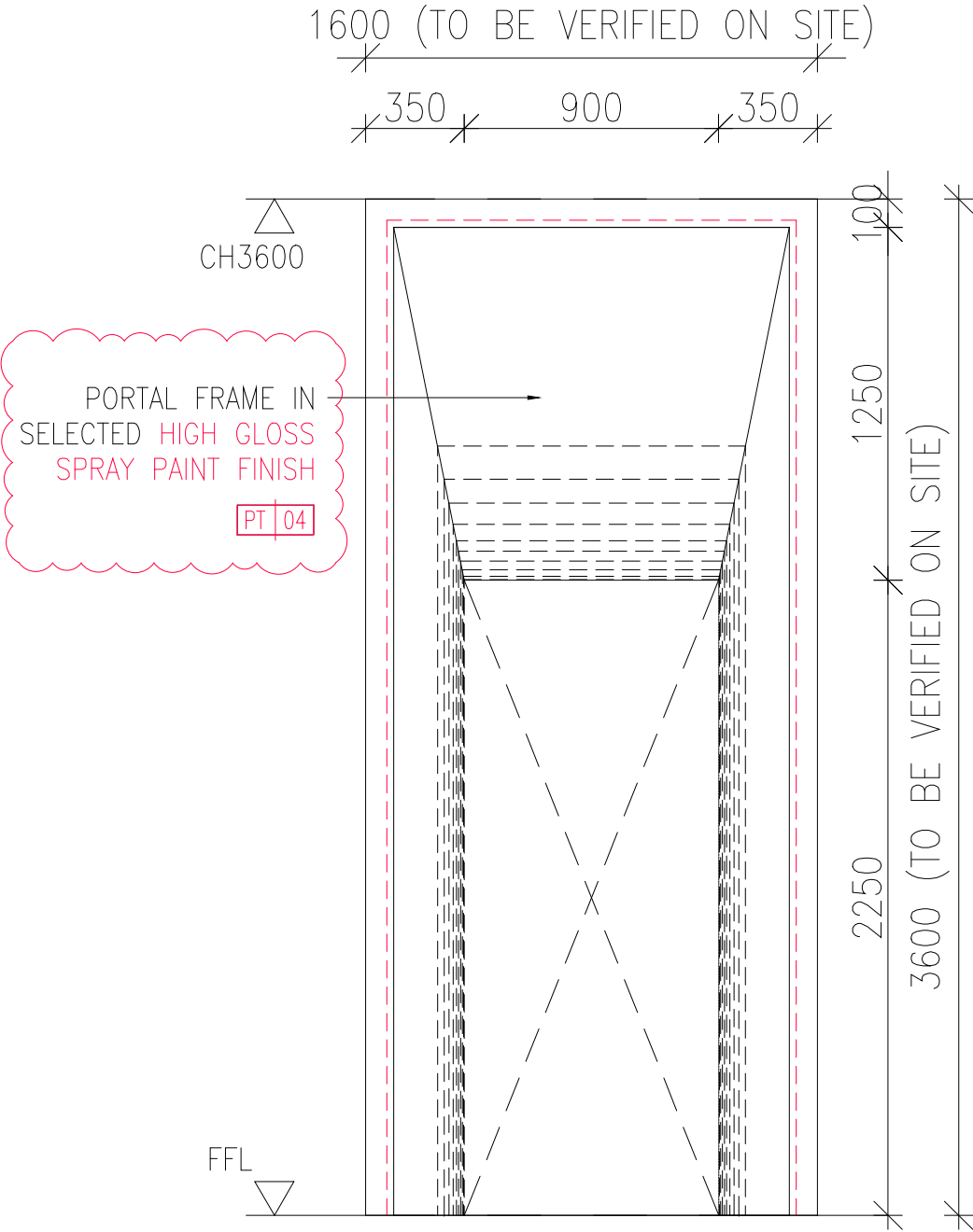
01 402 INSTAGRAM CORNER ELEVATION 2 SCALE 1:25
