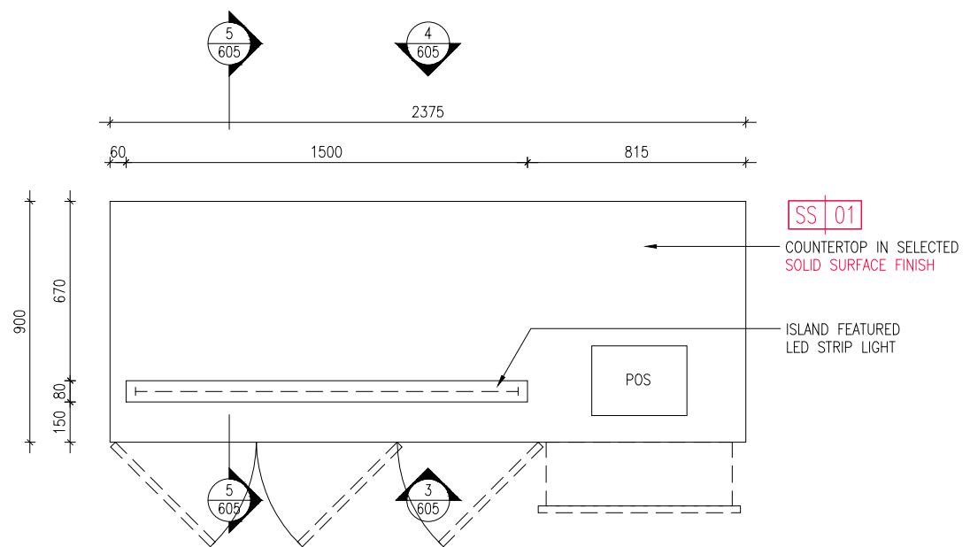
01 605 CAFÉ - FEATURE ISLAND - PART PLAN SCALE 1:25
