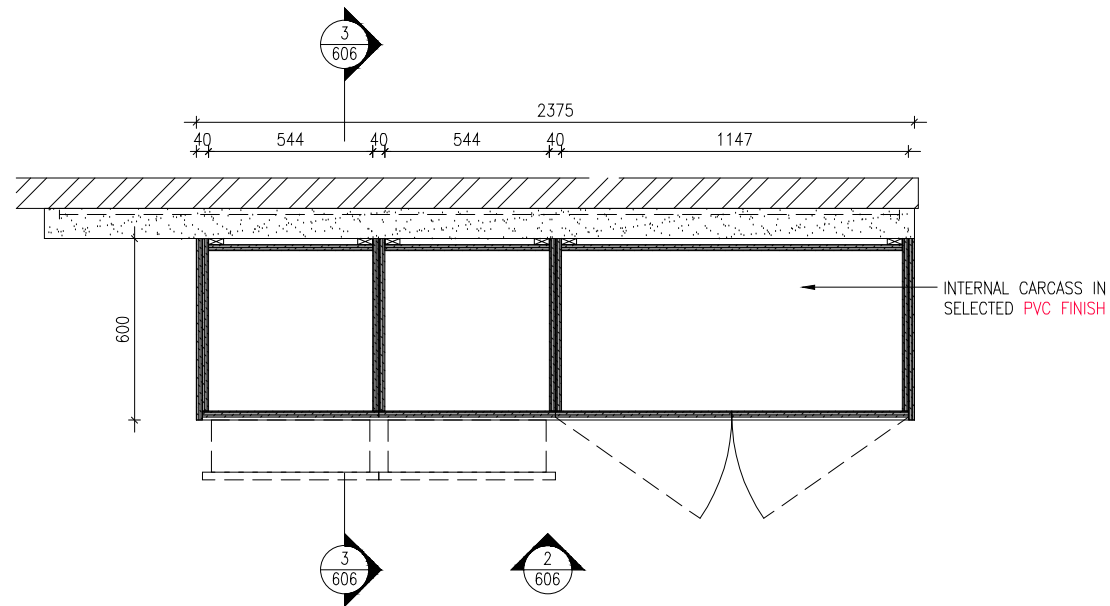
01 606 CAFÉ WORKING COUNTER - SECTIONAL PLAN VIEW SCALE 1:25
