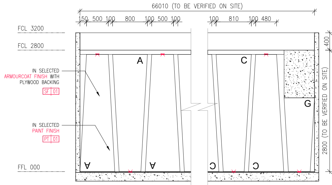
2 ELEVATION DETAIL 802 SCALE 1:50
