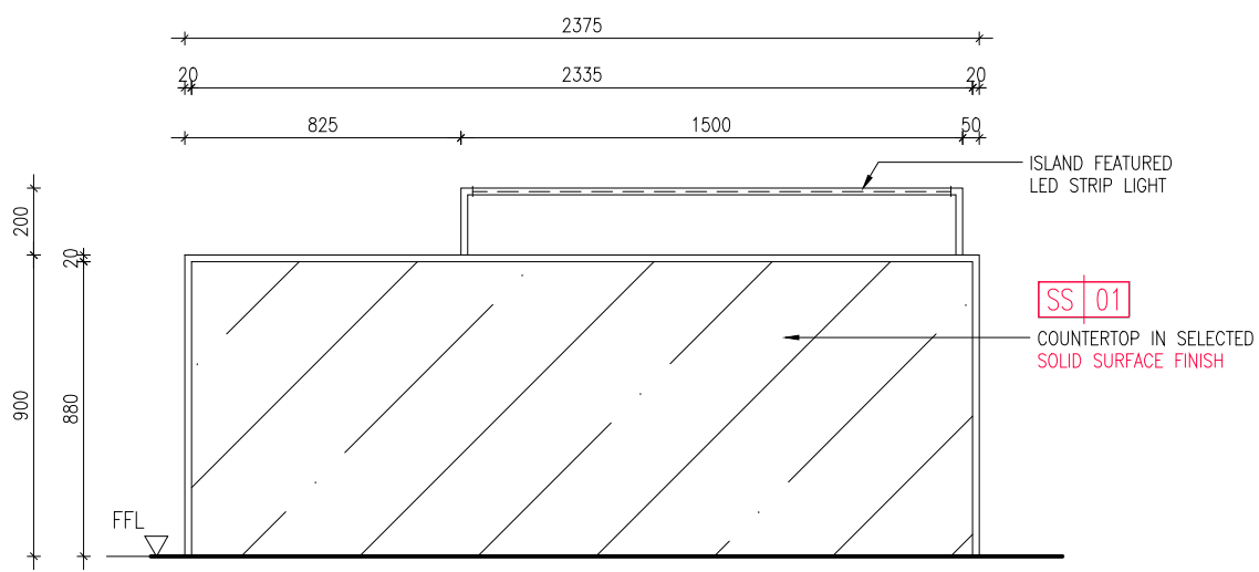
03 605 CAFÉ - FEATURE ISLAND - ELEVATION 1 SCALE 1:25
