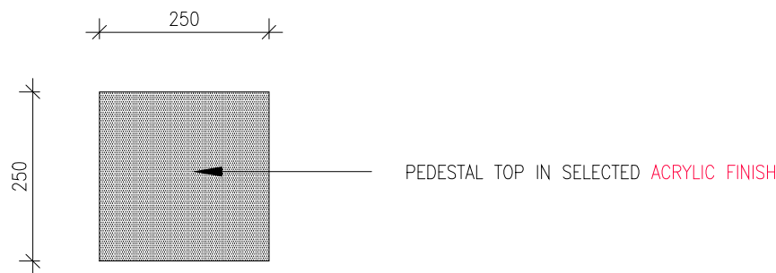
04 301 STAIRCASE PEDESTAL D - PLAN SCALE 1:10
