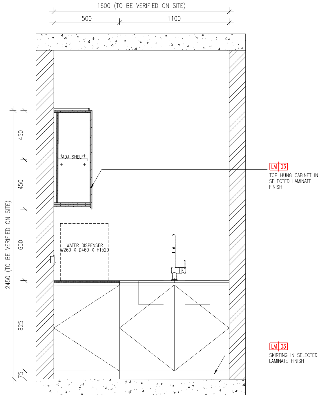
01 PANTRY ELEVATION 2 (EXTERNAL) 1102 SCALE 1:20
