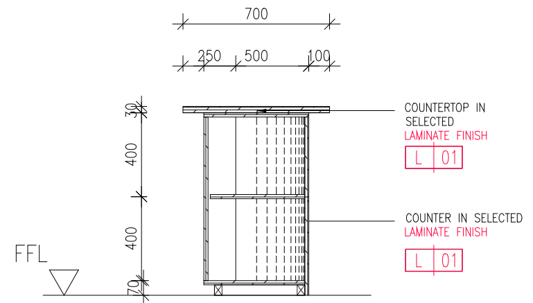
03 PRO SHOP COUNTER - ELEVATION 3 511 SCALE 1:25
