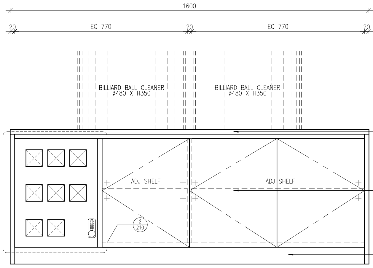
01 BILLIARD BALL CLEANER CABINET - FRONT 210 SCALE 1:10
