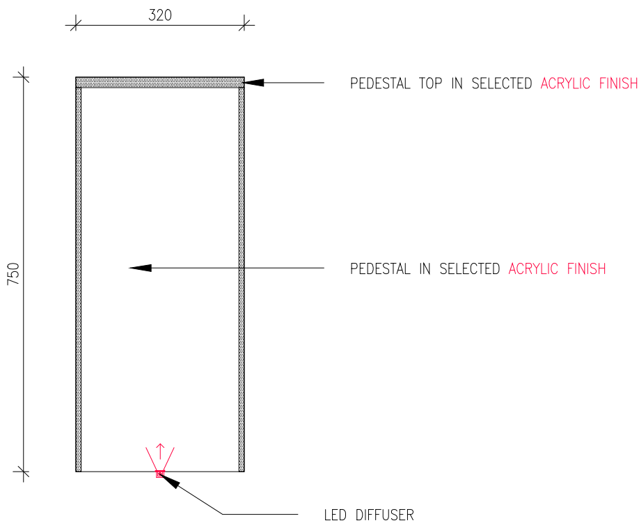
01 301 STAIRCASE PEDESTAL B - ELEVATION SCALE 1:10
