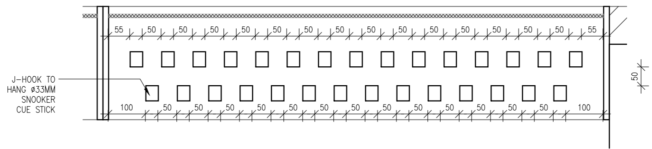
02 500 SNOOKER CUE STICK LOCATION SCALE 1:10
