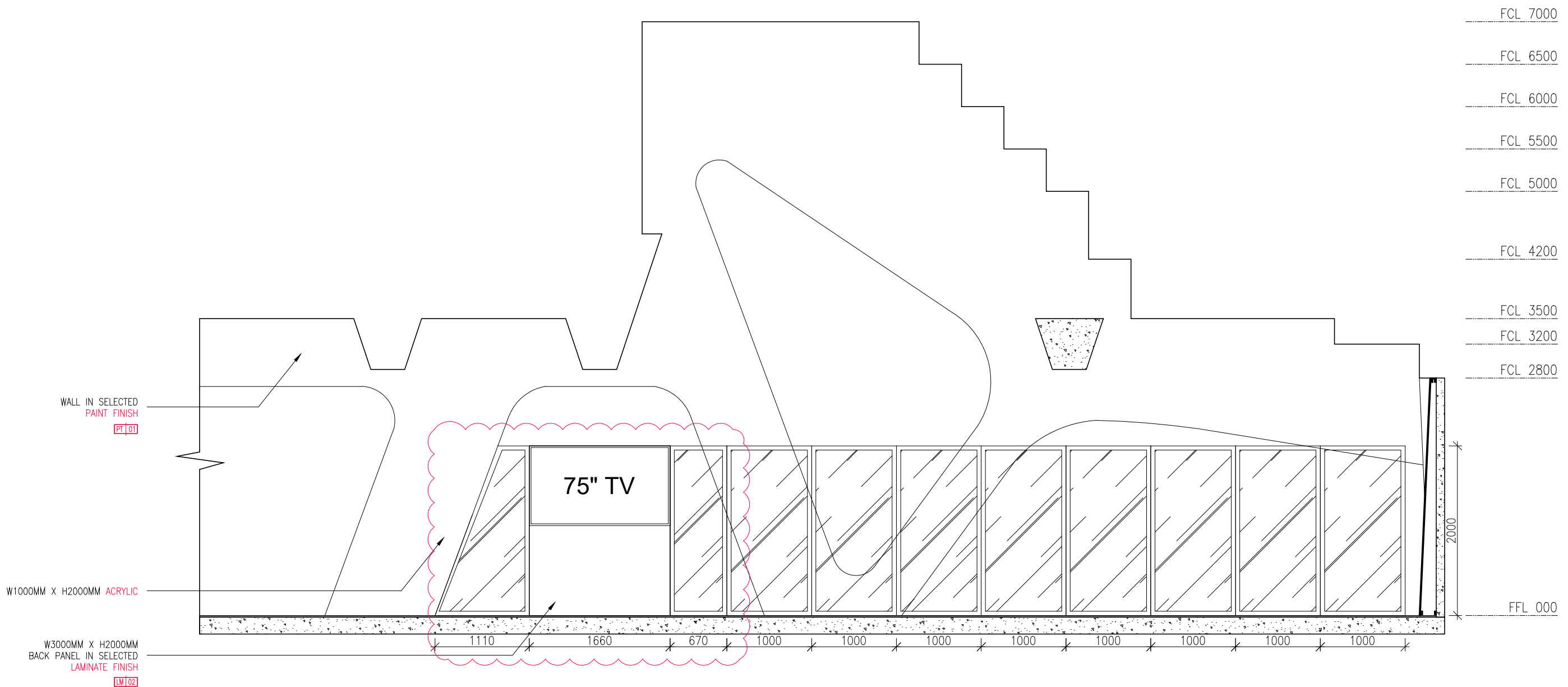
01 701 MEMBERS' LOUNGE ELEVATION 1:50
