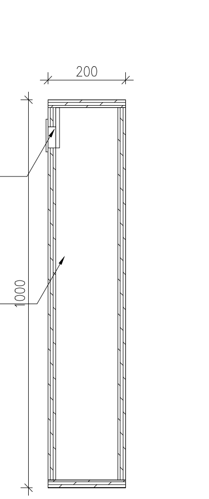
5 LOCKER B SIDE 1001 SCALE 1:10
