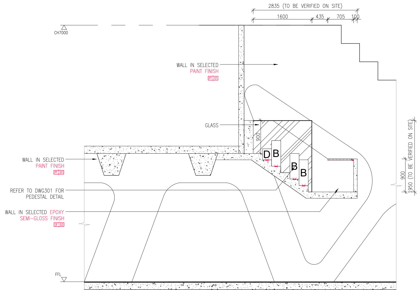
01 1303 STAIRCASE SECTION 3 SCALE 1:50
