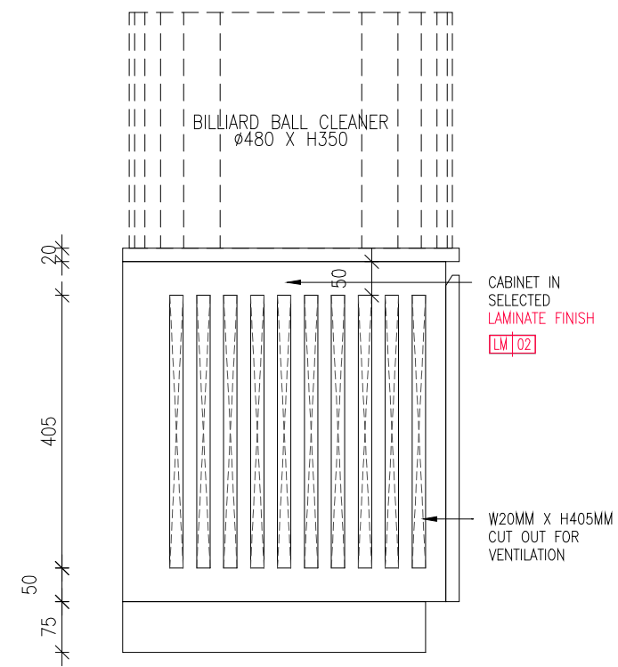
04 CABINET - SIDE ELEVATION 209 SCALE 1:5
