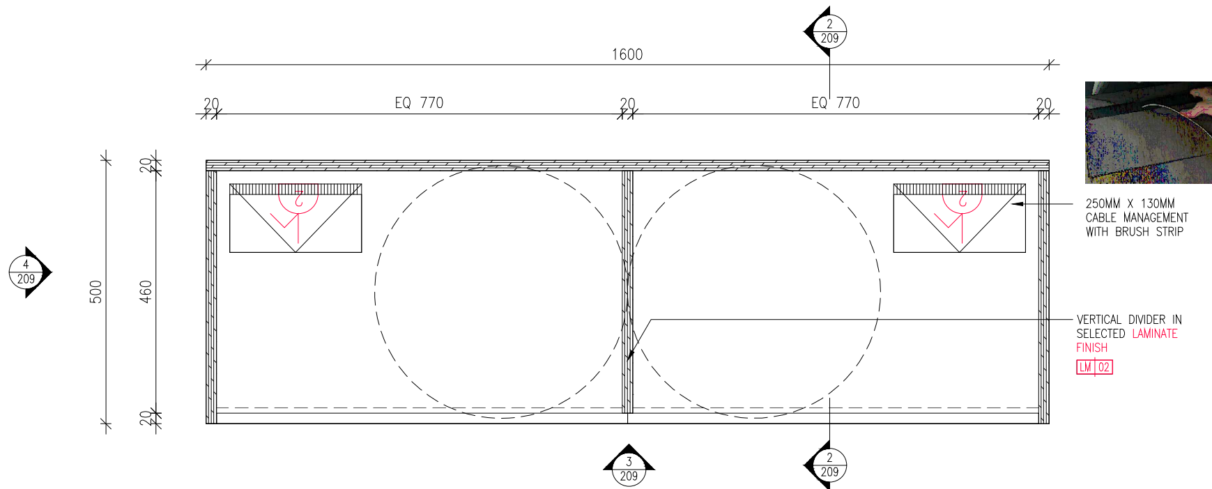
01 BILLIARD BALL CLEANER CABINET - PLAN 209 SCALE 1:10
