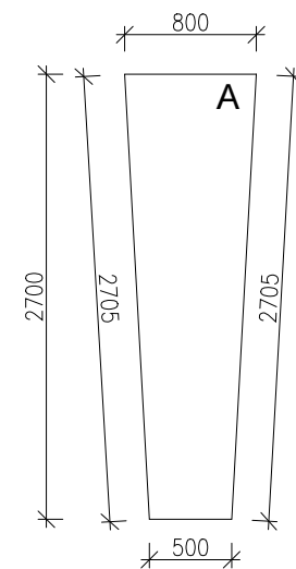
4 PANEL A 802 SCALE 1:50
