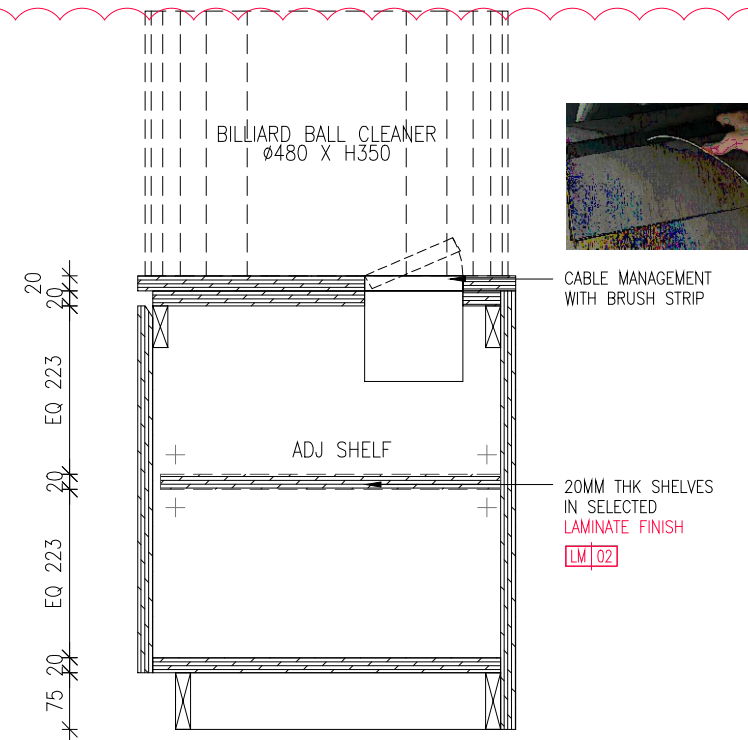
02 BILLIARD BALL CLEANER CABINET - SECTION 209 SCALE 1:10
