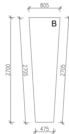
5 PANEL B 802 SCALE 1:50
