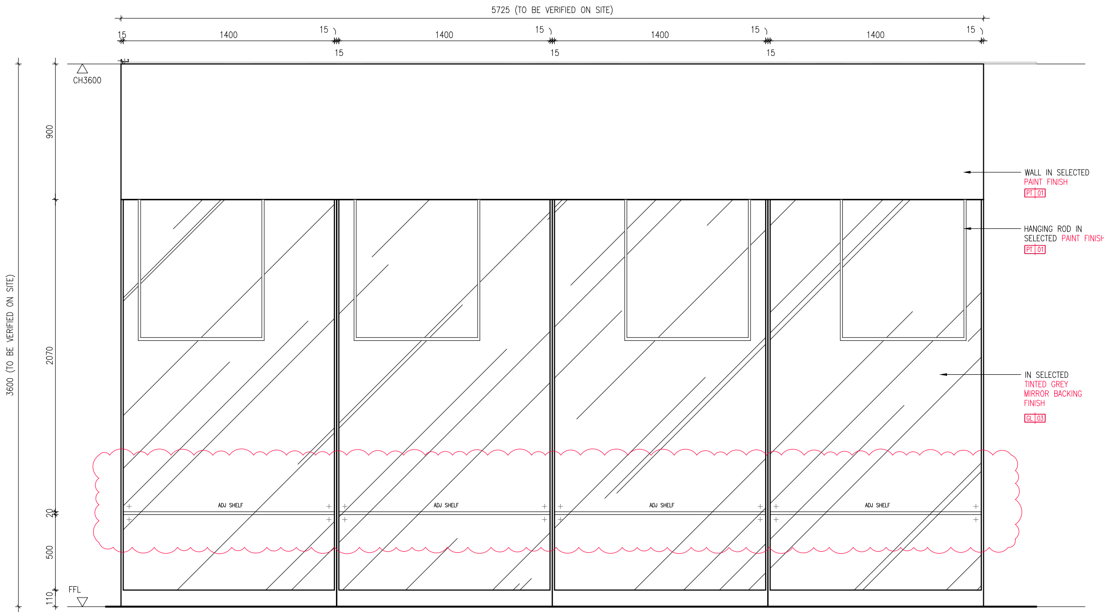
02 300 MERCHANDISE DISPLAY - ELEVATION SCALE 1:25
