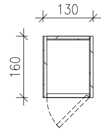
3 LOCKER C PLAN 1002 SCALE 1:10
