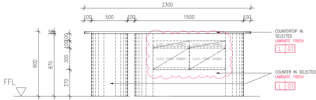
01 PRO SHOP COUNTER - ELEVATION 1 511 SCALE 1:25
