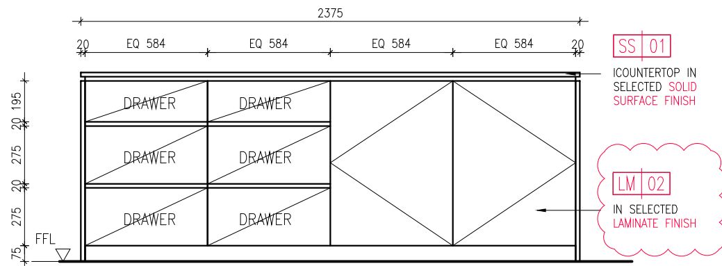
02 606 CAFÉ WORKING COUNTER - ELEVATION 1 SCALE 1:25
