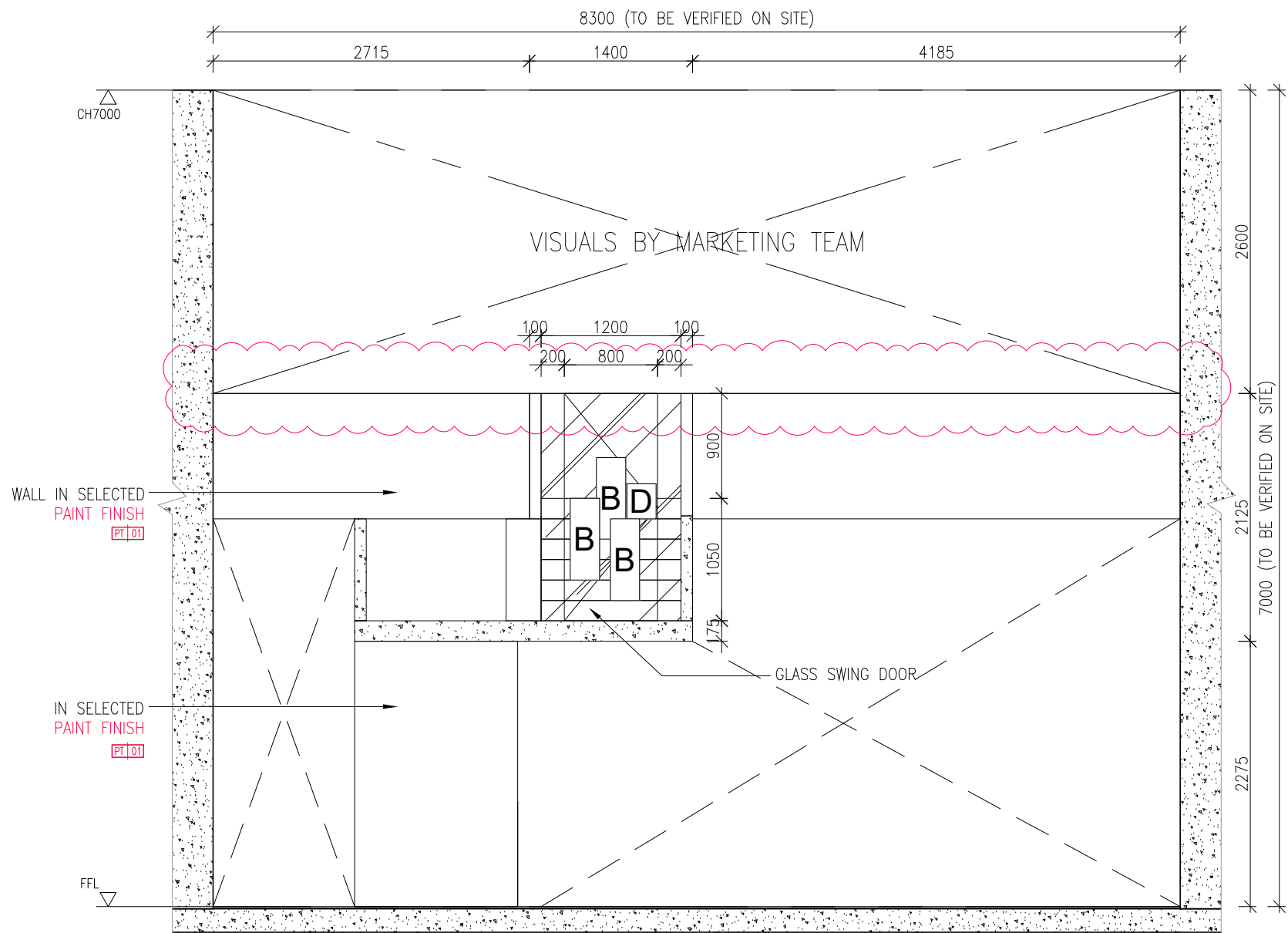
01 1301 STAIRCASE SECTION 1 SCALE 1:50
