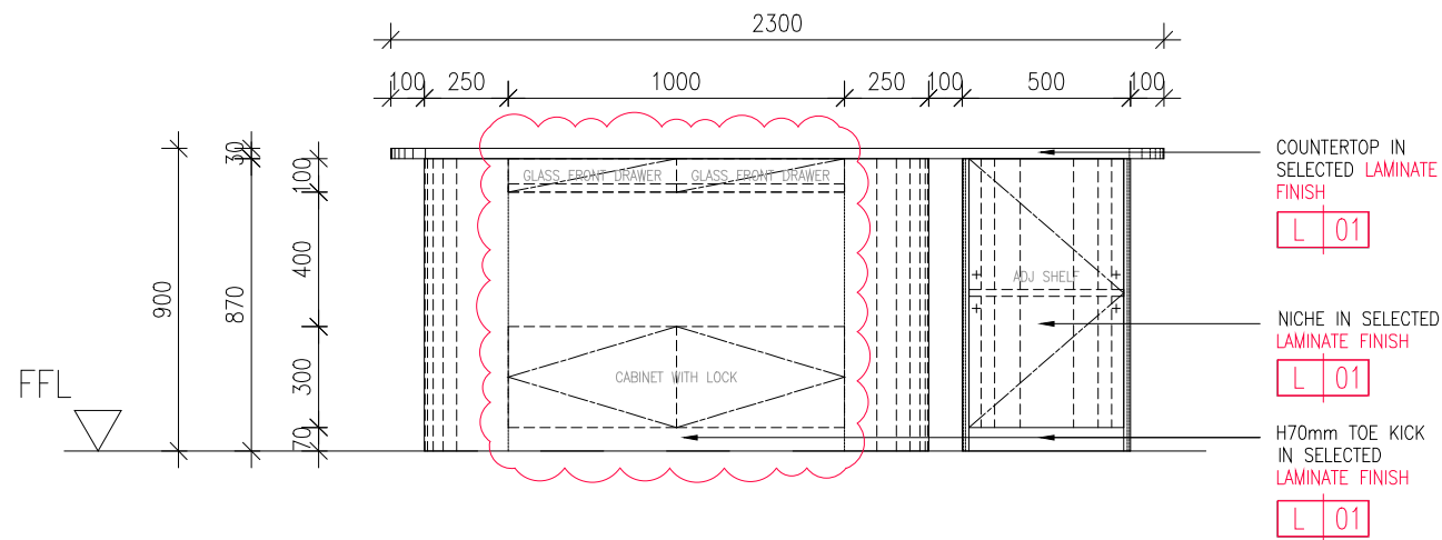
02 PRO SHOP COUNTER - ELEVATION 2 511 SCALE 1:25
