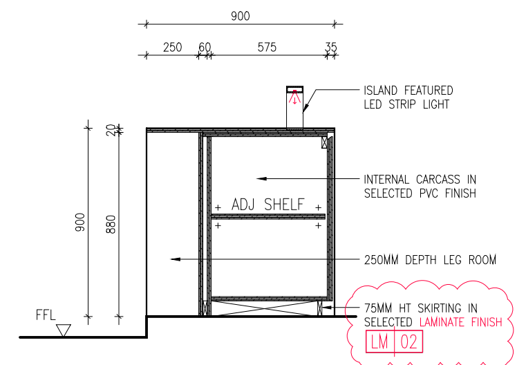
05 605 CAFÉ - FEATURE ISLAND - SECTION SCALE 1:25
