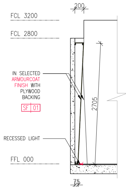
3 SECTION DETAIL 802 SCALE 1:50
