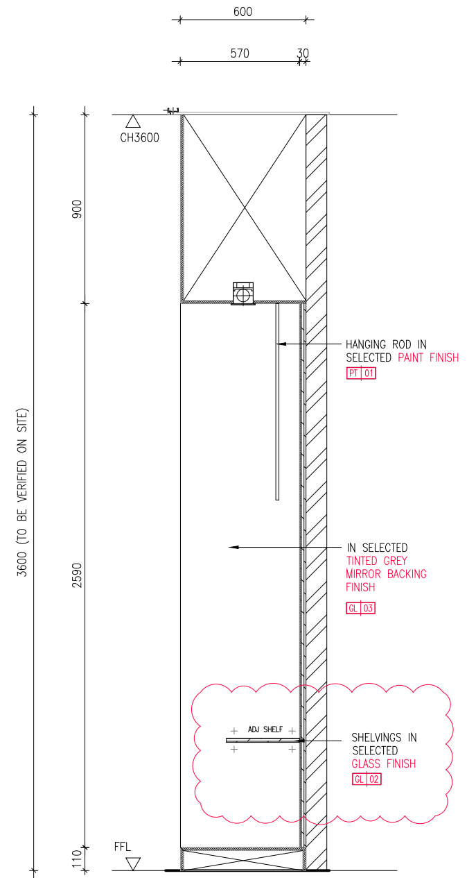
03 300 MERCHANDISE DISPLAY - SECTION SCALE 1:25
