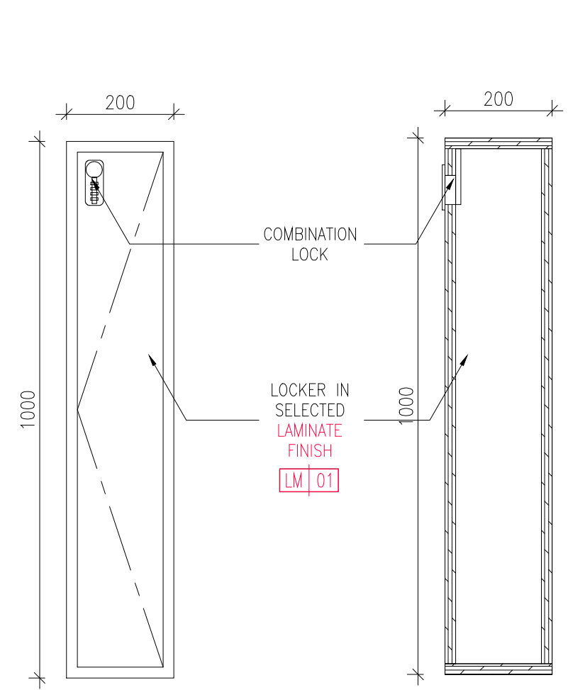
4 LOCKER B FRONT 1001 SCALE 1:10
