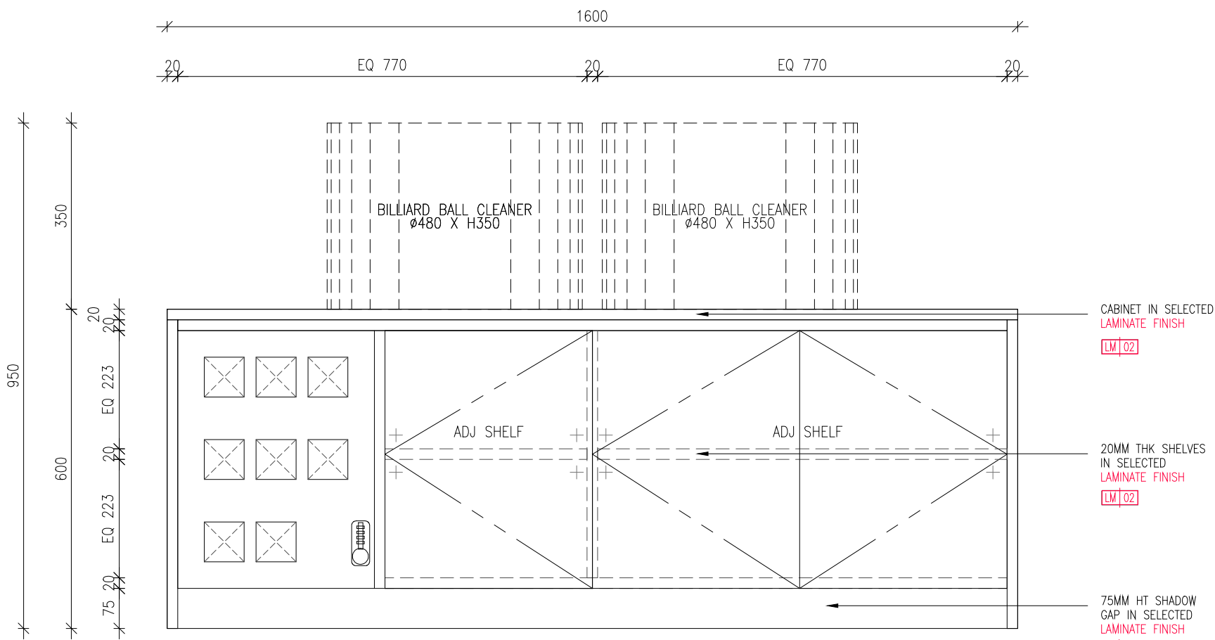
03 BILLIARD BALL CLEANER CABINET - FRONT 209 SCALE 1:10
