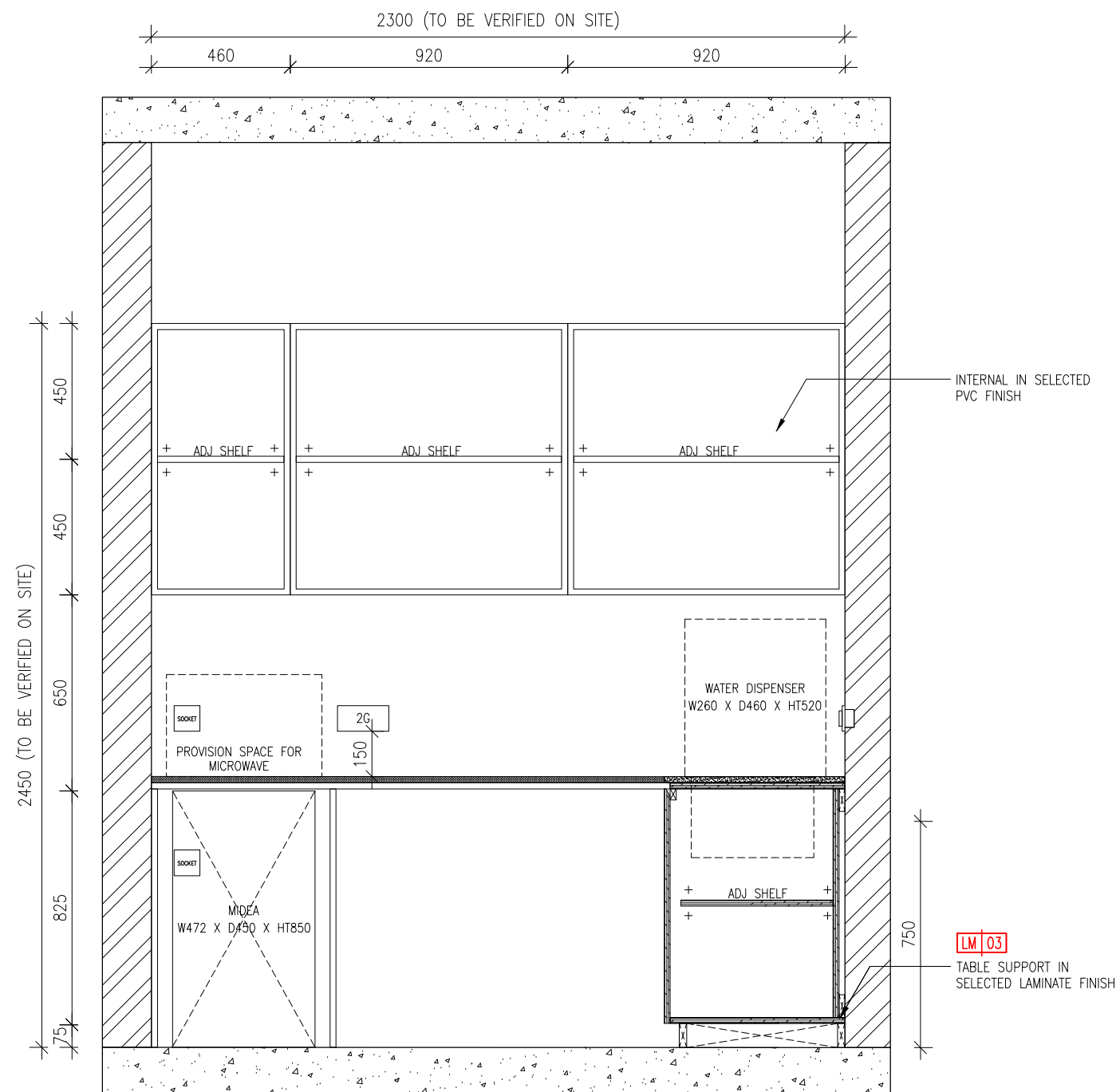
02 PANTRY ELEVATION 1 (INTERNAL) 1101 SCALE 1:20
