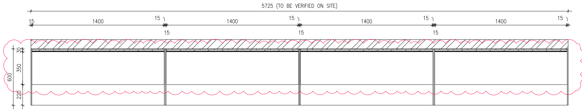
01 300 MERCHANDISE DISPLAY - PART PLAN SCALE 1:25
