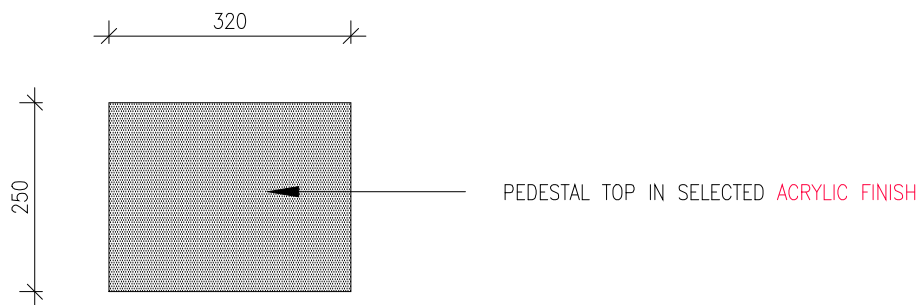
03 301 STAIRCASE PEDESTAL B - PLAN SCALE 1:10
