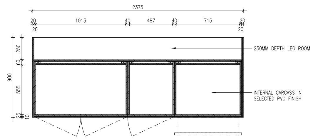
02 605 CAFÉ - FEATURE ISLAND - SECTIONAL PART PLAN SCALE 1:25
