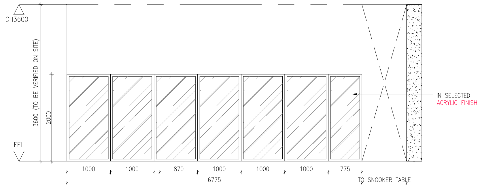
01 702 MEMBERS' LOUNGE ELEVATION 1:50
