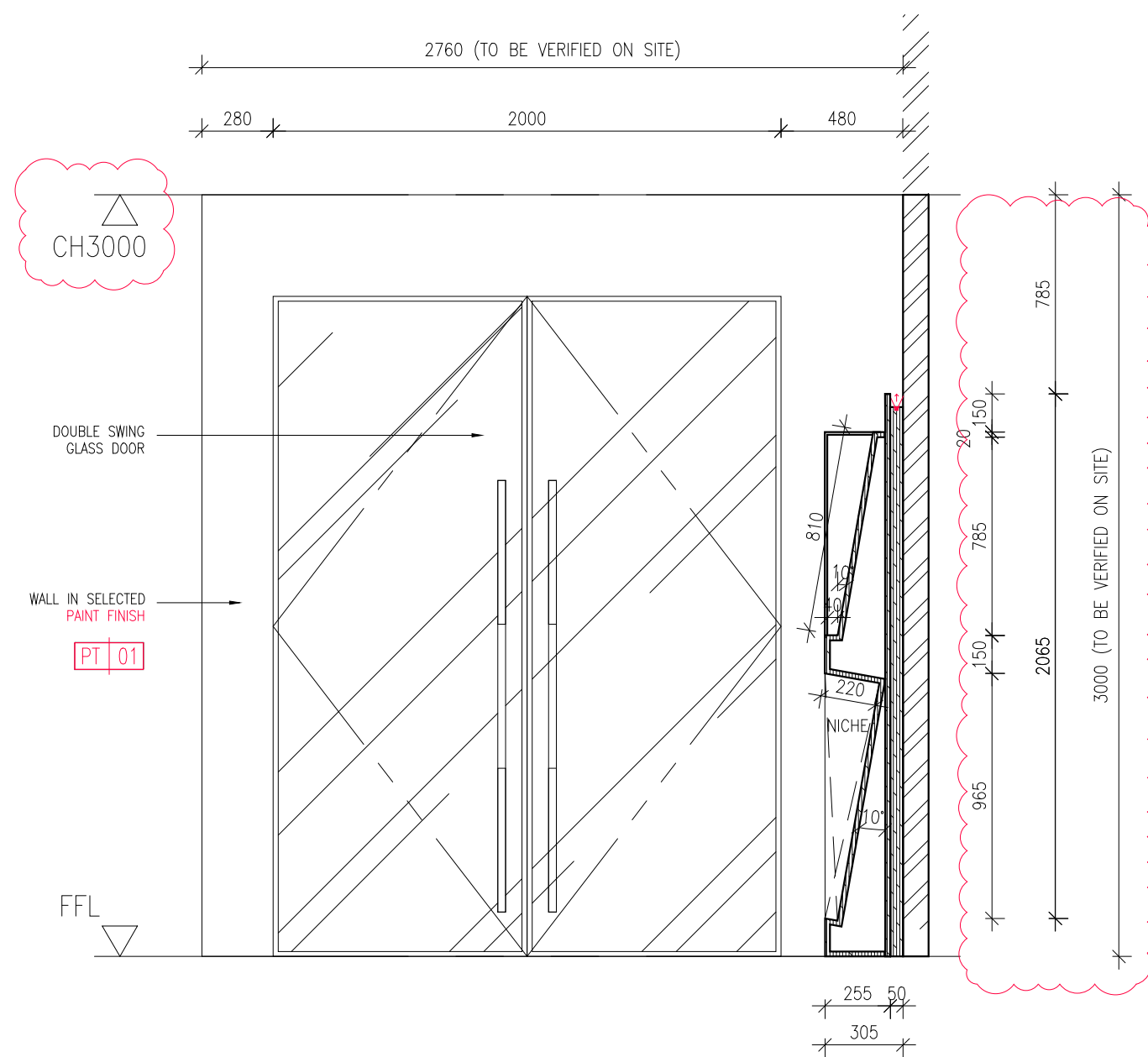
01 503 PRO SHOP - ELEVATION 3 SCALE 1:25
