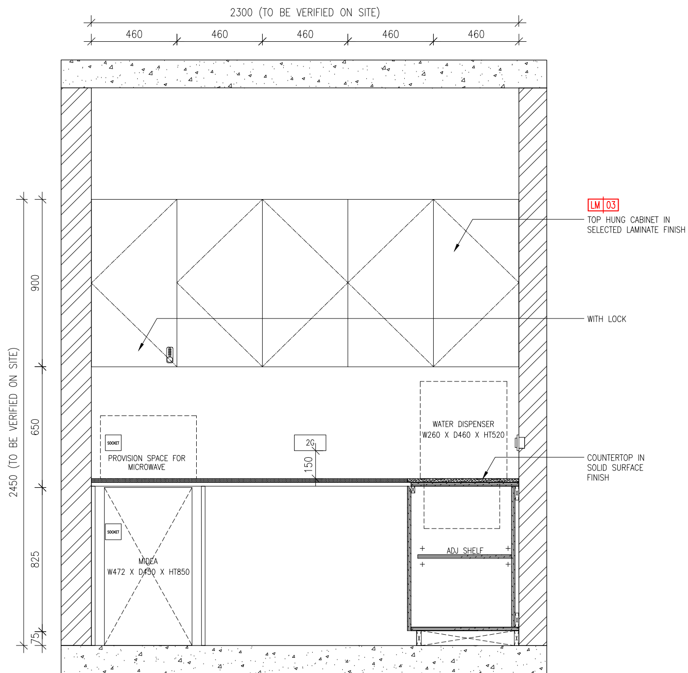
01 PANTRY ELEVATION 1 (EXTERNAL) 1101 SCALE 1:20
