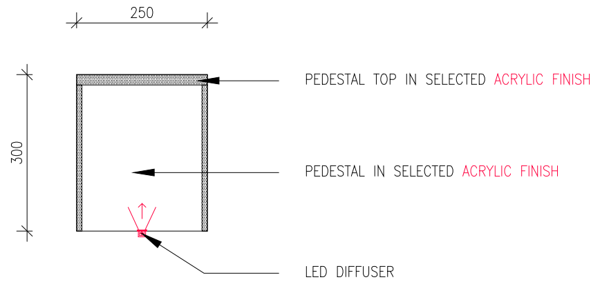
02 301 STAIRCASE PEDESTAL D - ELEVATION SCALE 1:10
