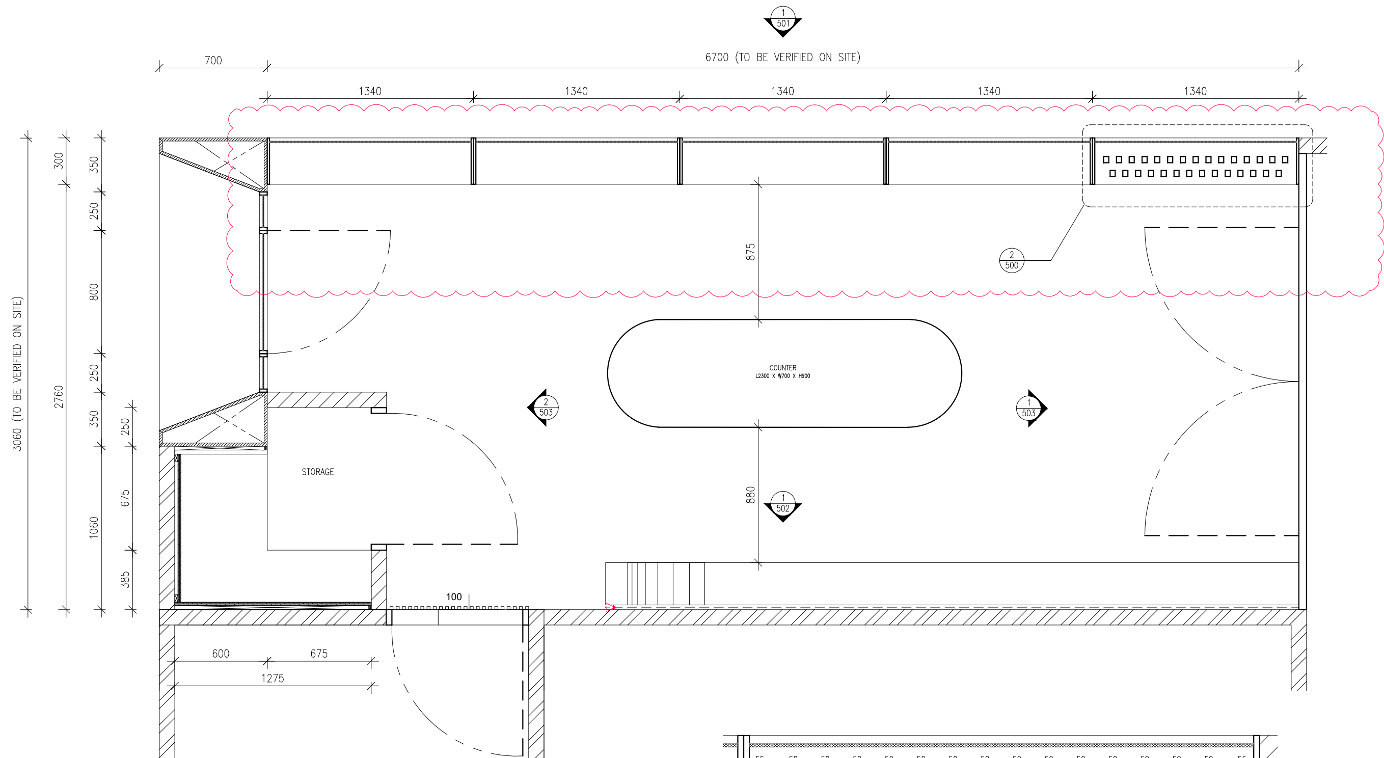
01 500 PRO SHOP - PART PLAN SCALE 1:25
