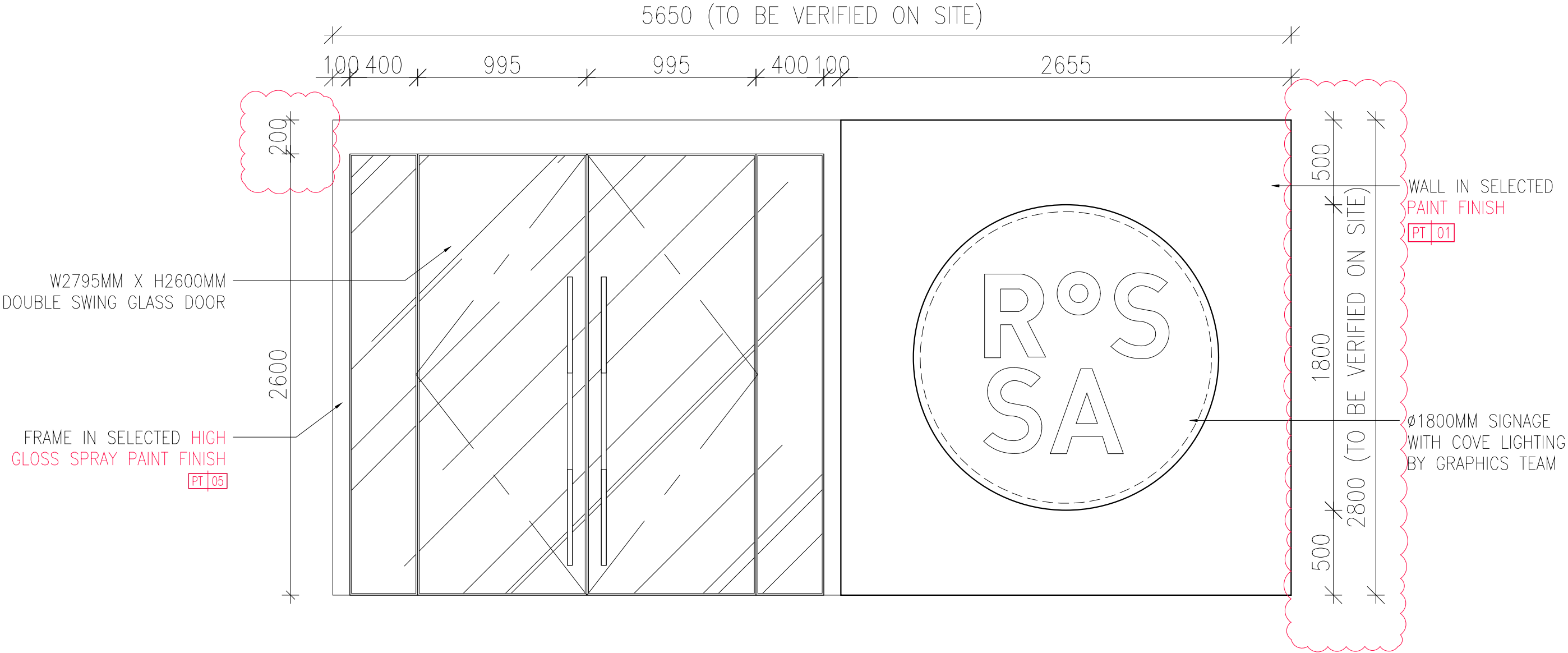
01 207 ENTRANCE - ELEVATION SCALE 1:25
