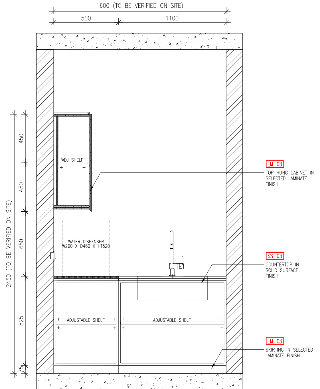
02 PANTRY ELEVATION 2 (INTERNAL) 1102 SCALE 1:20
