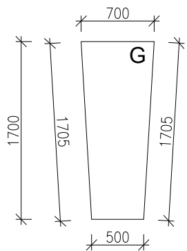
7 PANEL G 802 SCALE 1:50
