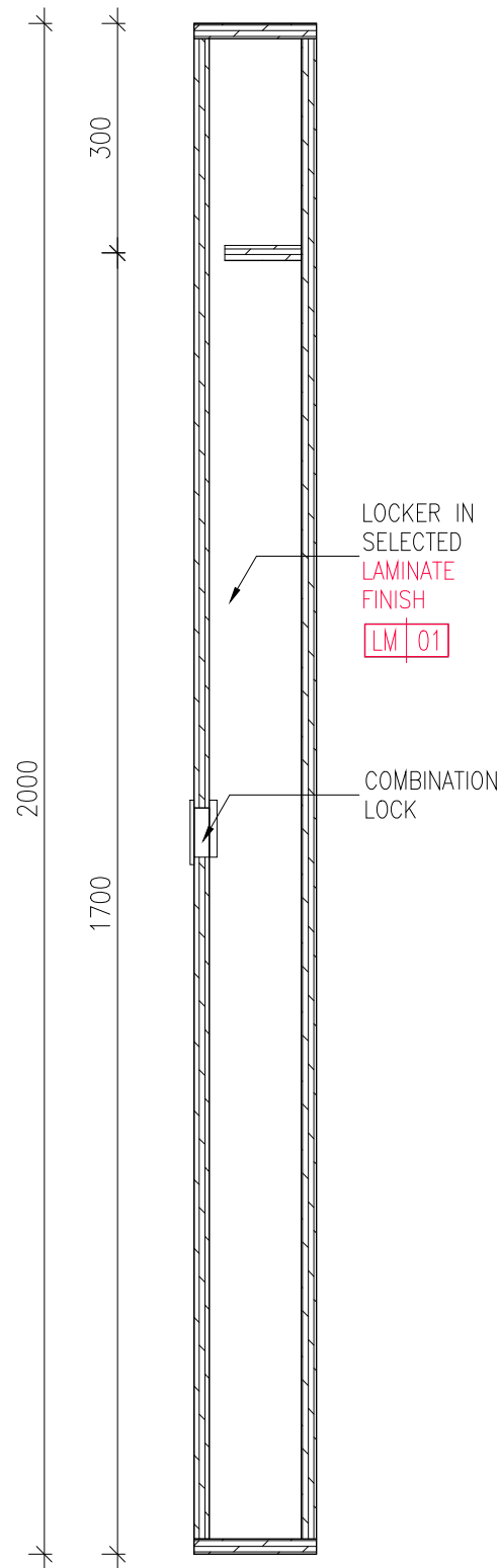
2 LOCKER C SIDE 1002 SCALE 1:10
