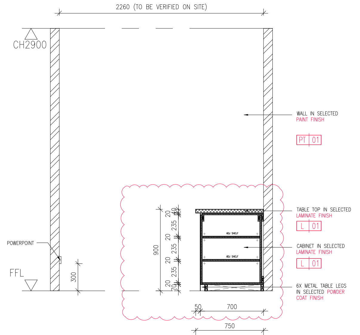
02 EQUIPMENT SERVICING ROOM - SECTION SCALE 1:25
