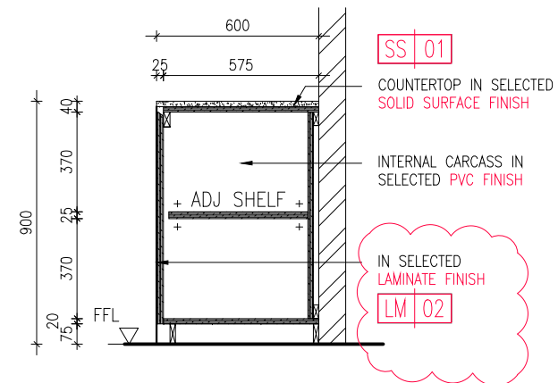
03 606 CAFÉ WORKING COUNTER - SECTION SCALE 1:25
