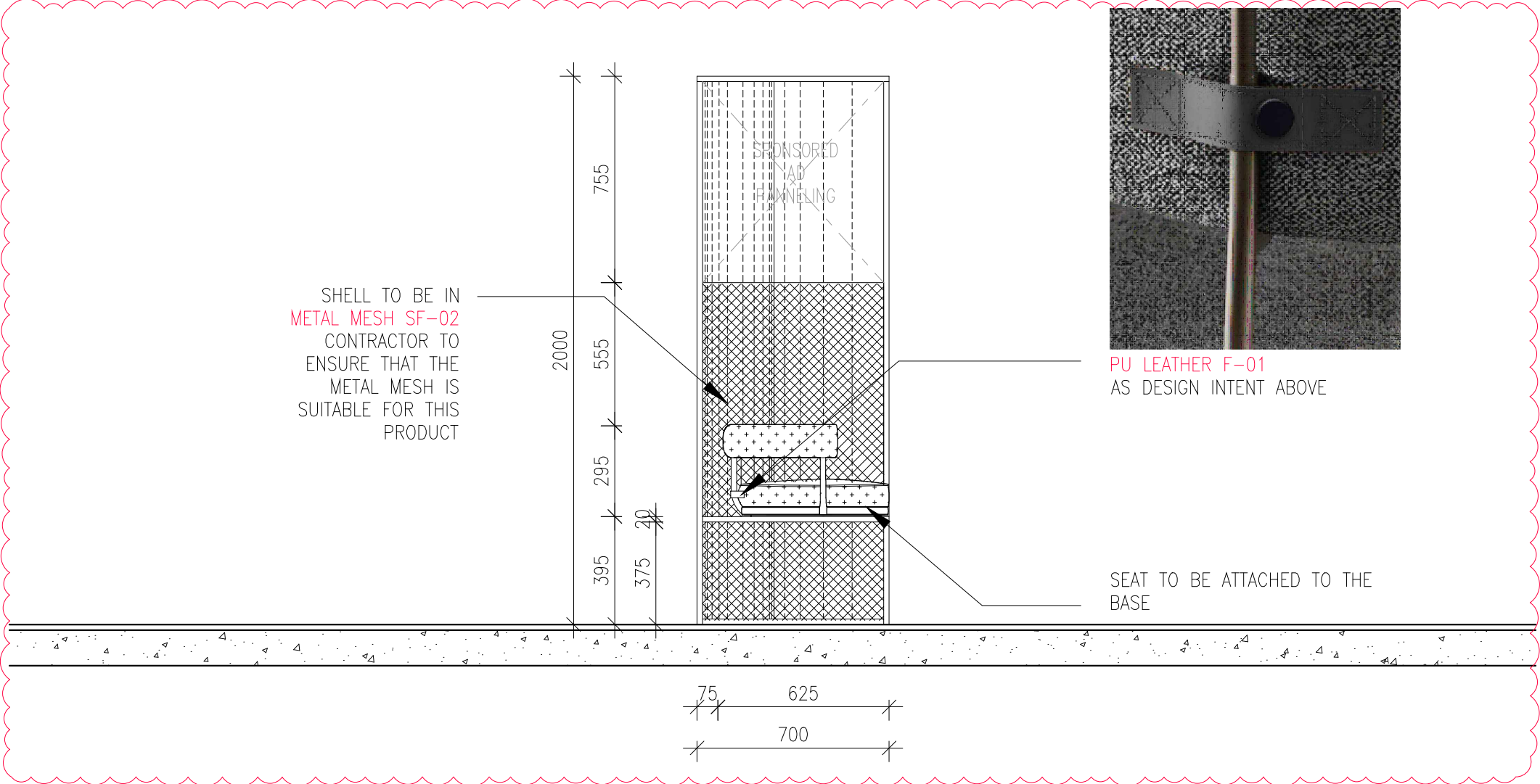
01 SEATING (TOURNAMENT) SECTION 923 SCALE 1:20
