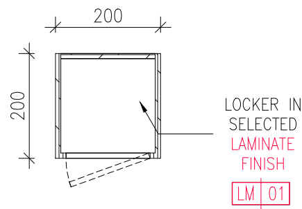
6 LOCKER A & B PLAN 1001 SCALE 1:10
