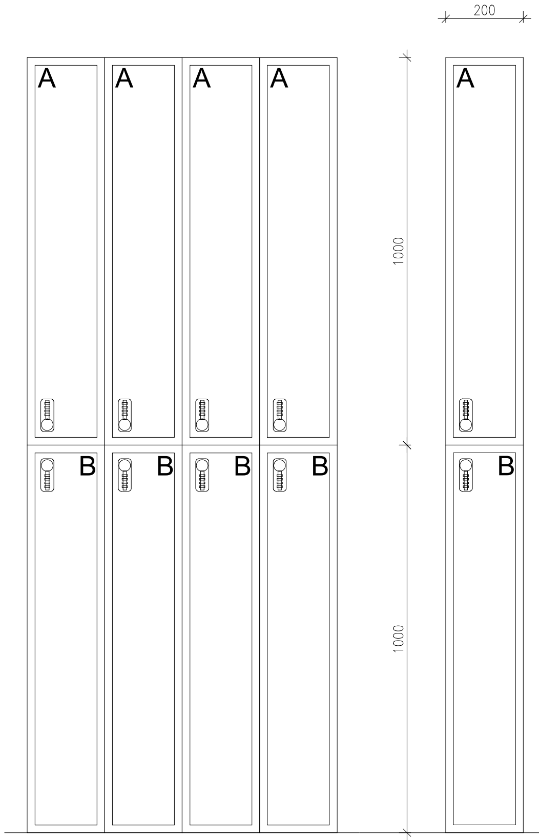
1 FRONT ELEVATION 1001 SCALE 1:10
