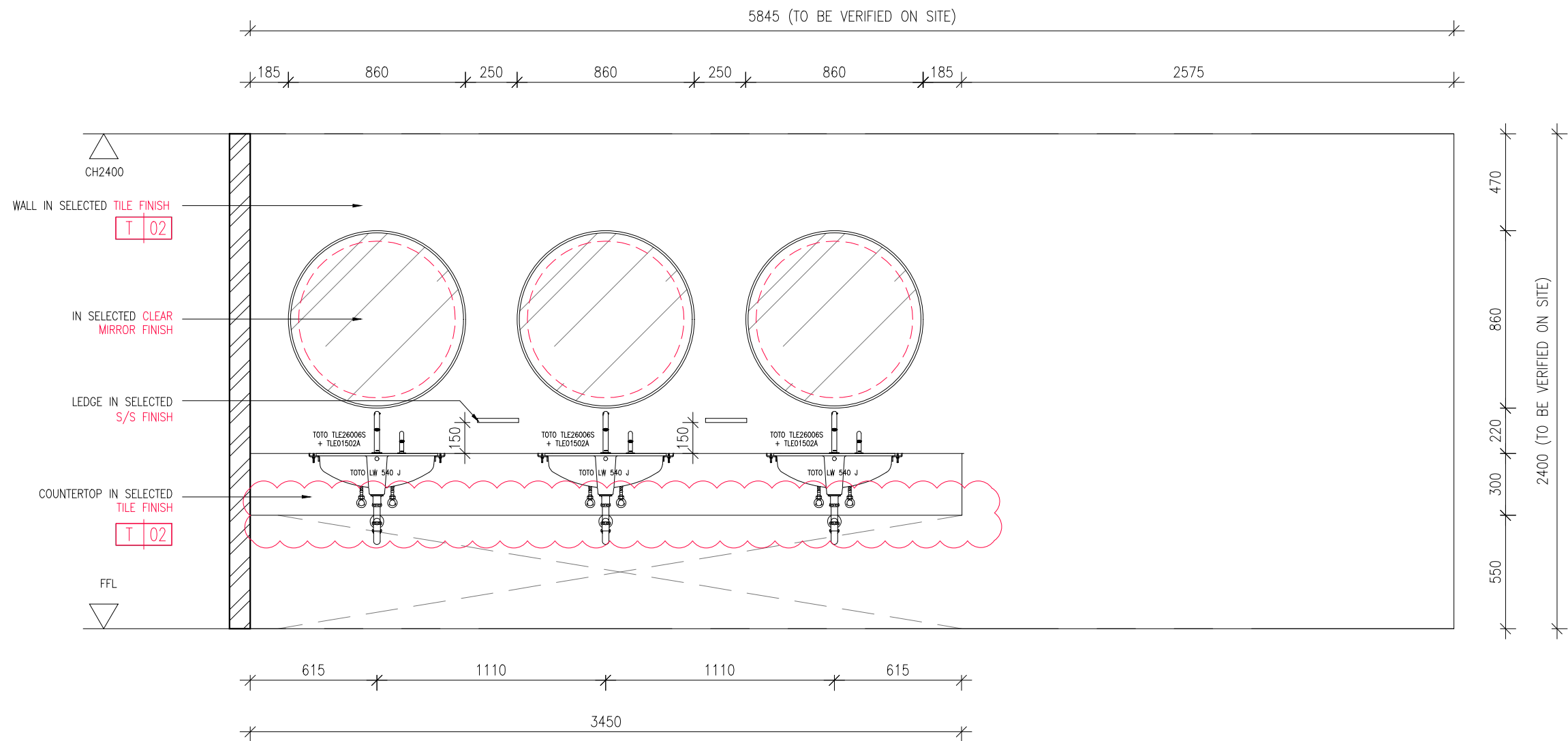
01 1201 FEMALE TOILET ELEVATION 1 1:25
