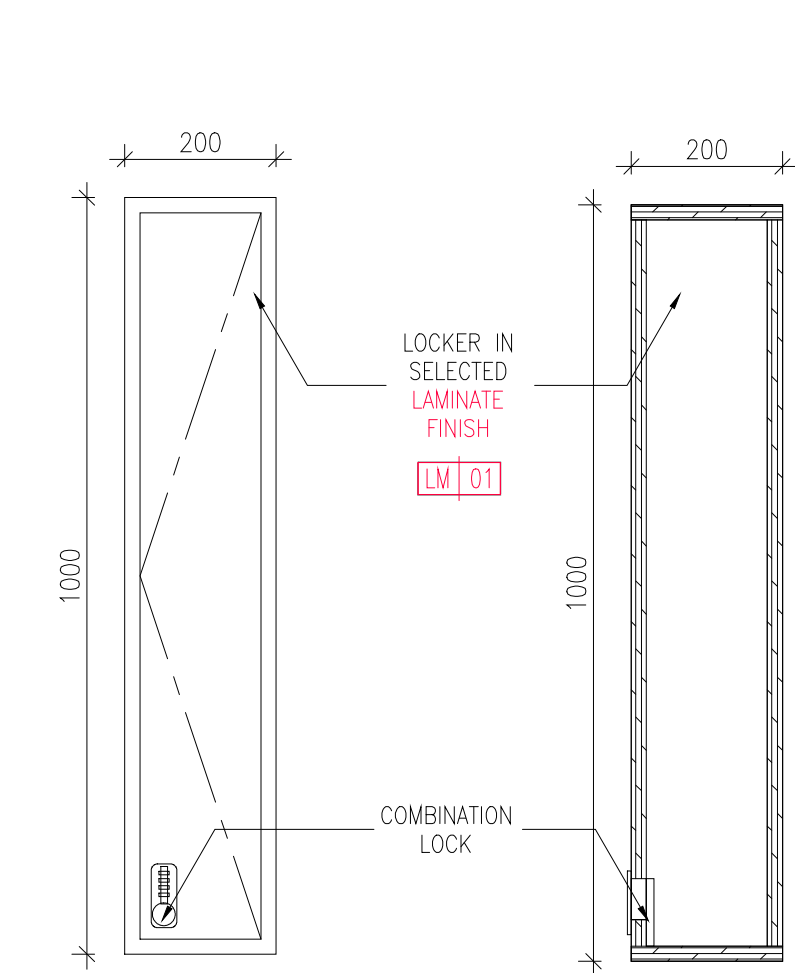
2 LOCKER A FRONT 1001 SCALE 1:10
