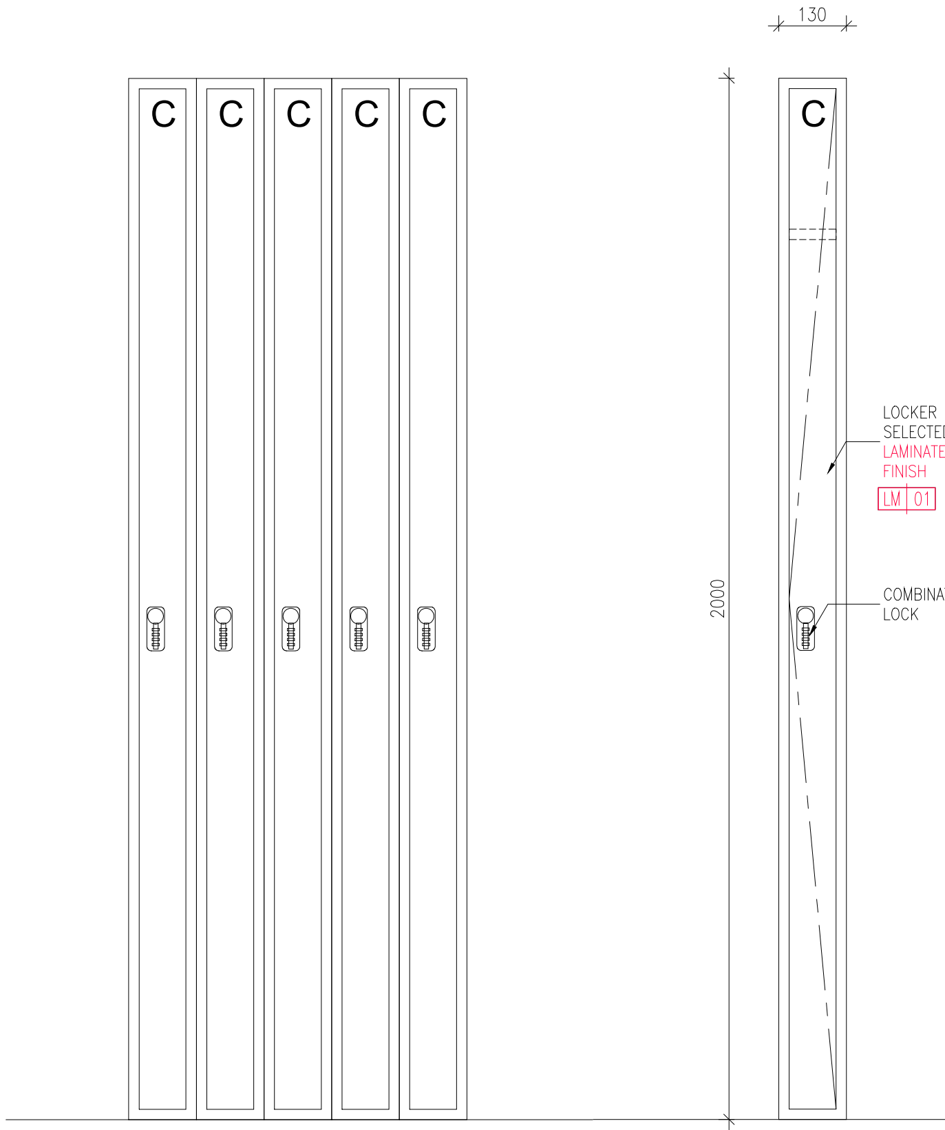
1 FRONT ELEVATION 1002 SCALE 1:10
