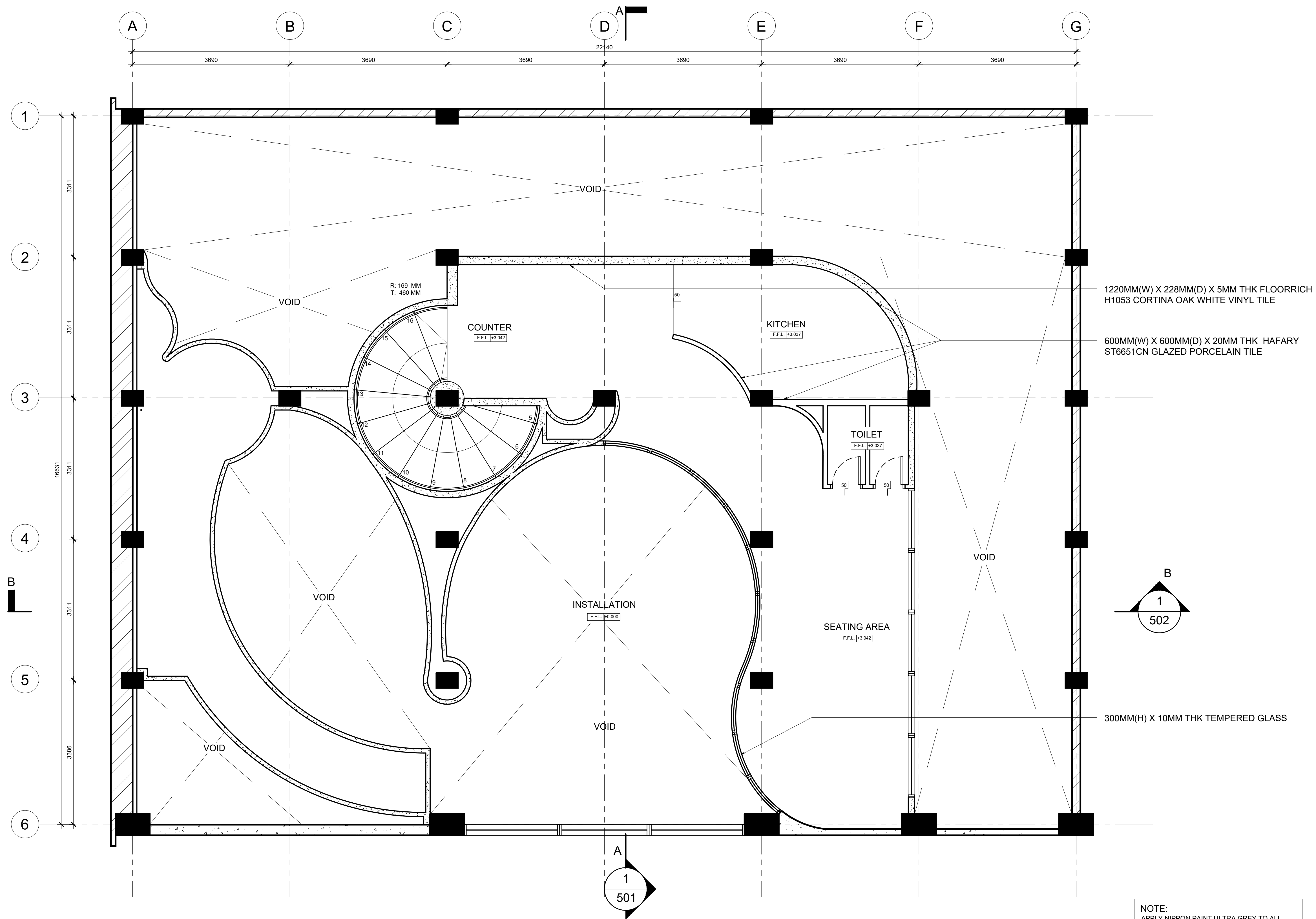
1 304 WALL FINISHES PLAN - LEVEL 2 SCALE : 1 : 50
