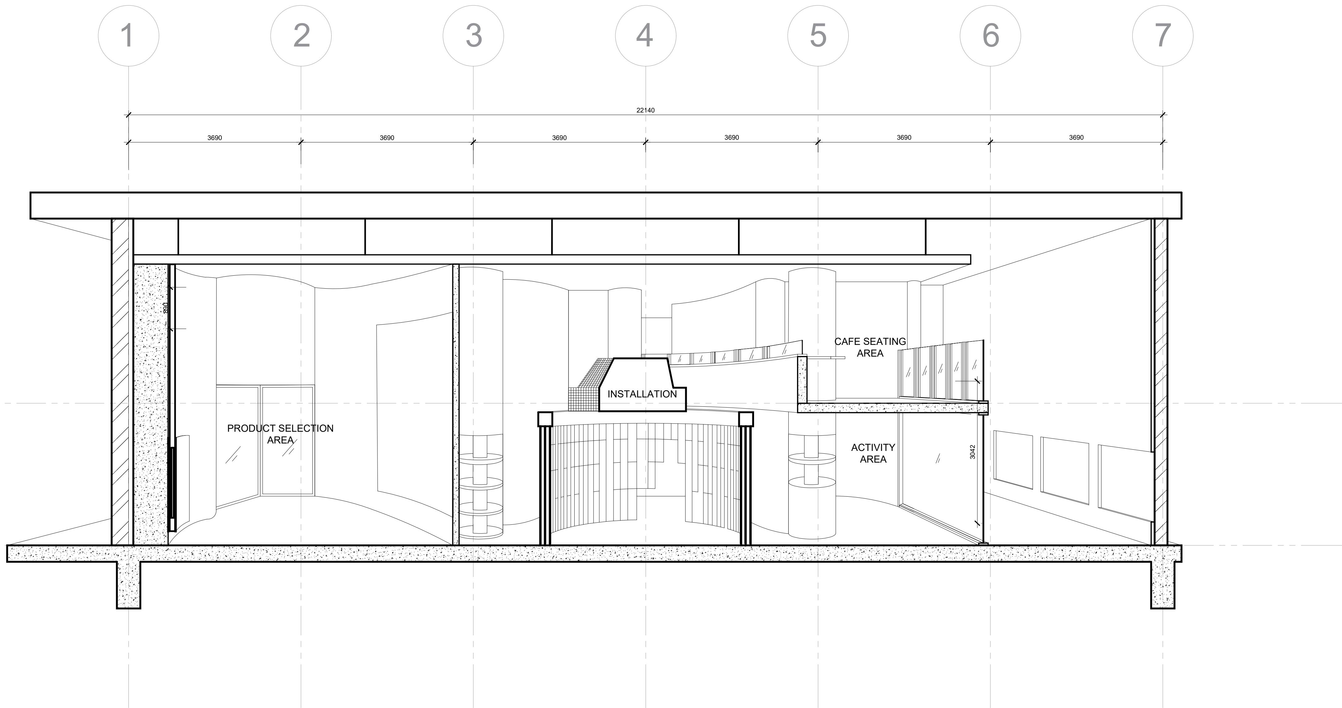
SECTIONAL PERSPECTIVE B-B SCALE : 1 : 50
